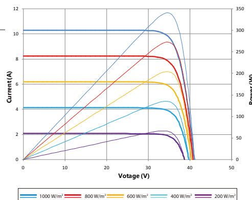
Current-Voltage & Power-Voltage Curve (340S)
