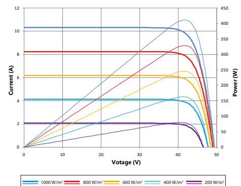
Current-Voltage & Power-Voltage Curve (410S)
